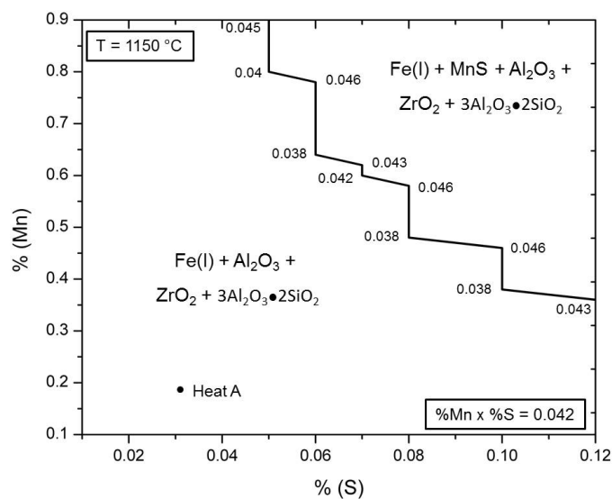
Fig. 9. Stability phase diagram of heat A to different Mn and S contents at 1150°C. Values represent the factor %Mn × %S to different Mn and S contents and it shows the %Mn × %S average value. The solid circle represents the chemical composition of Heat A
