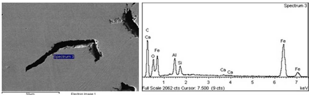
Fig. 7. SEM analysis of a graphite flake edge for heat B
