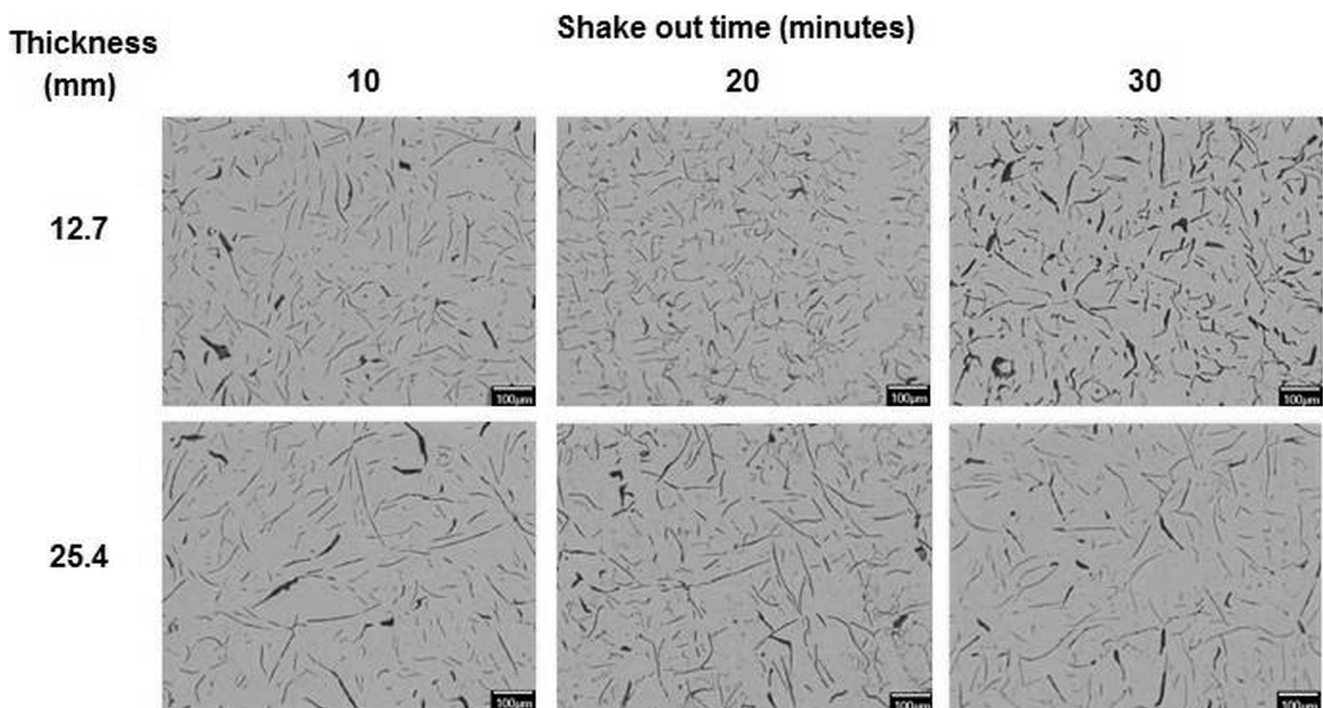
Fig. 3. Unetched microstructure for the 12.7 mm and 25.4 thickness plates after the shakeout time of 10 min., 20 min., and 30 min. of heat B
