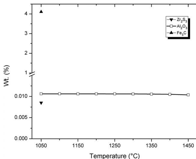
Fig. 12. Phases formed during the solidification of Heat B. Lines represent the weight % of each solid phase formed. The balance corresponds % liquid in the system at each temperature
