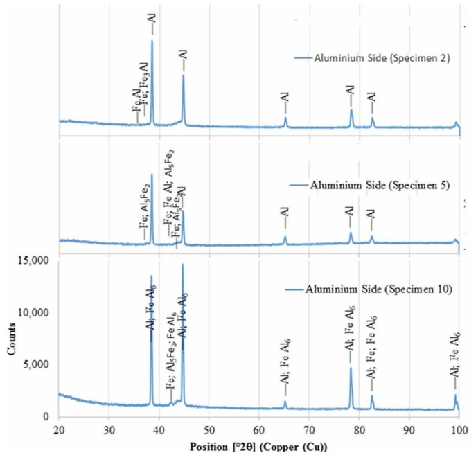
Fig. 6. XRD Analysis of the aluminum side of the specimens' fracture surfaces after ram tests
