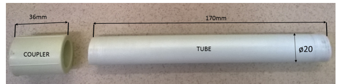
Fig. 1. Polypropylene components: tube after end milling and coupler fitted into a tube diameter
