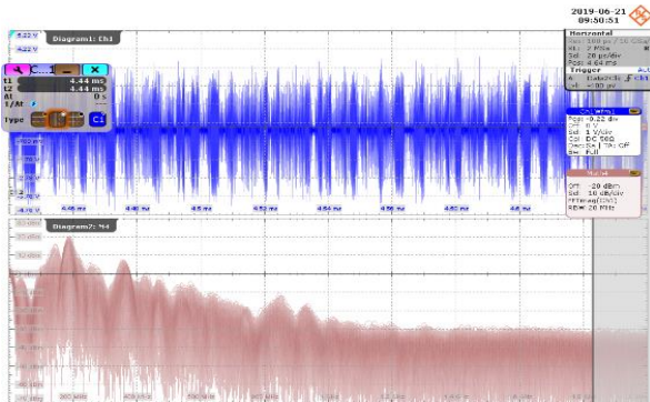
Fig 8: The oscillogram and spectrum of masking noise created by a noise generator
