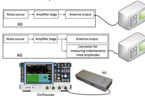
Fig. 3. Schematic of a measuring bench using a digital storage oscilloscope
