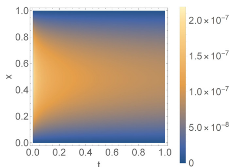
Fig. 5. The absolute error generated by the numerical method for the first example, \alpha = 0.25, \Delta x = \frac{1}{200}, \Delta t = \frac{1}{200}
