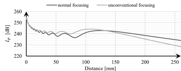
Fig. 13. Calculation results for the acoustic field distribution in the form of L_p(x) , y = 0 , with the number of activated transducers n = 64 for normal focusing and for unconventional focusing with a shift by \lambda .
