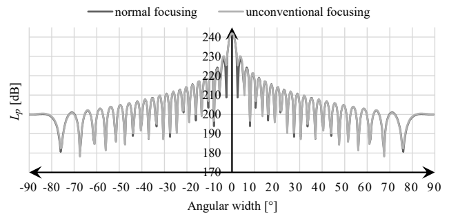
Fig. 10. Calculation results for the acoustic field distribution for the ring array in the form of L_p(x) with the number of activated transducers n = 64 for normal focusing and for unconventional focusing with a shift by \lambda/2 .
