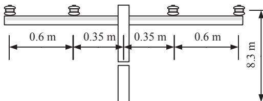
Fig. 1. Crossarm construction
