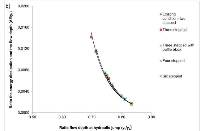
Fig. 3. Relationship between the Froude number and \Delta E/L_j (a); the relationship between y_1/y_2 and \Delta E/y_1 (b), for different weir steps; source: own study
