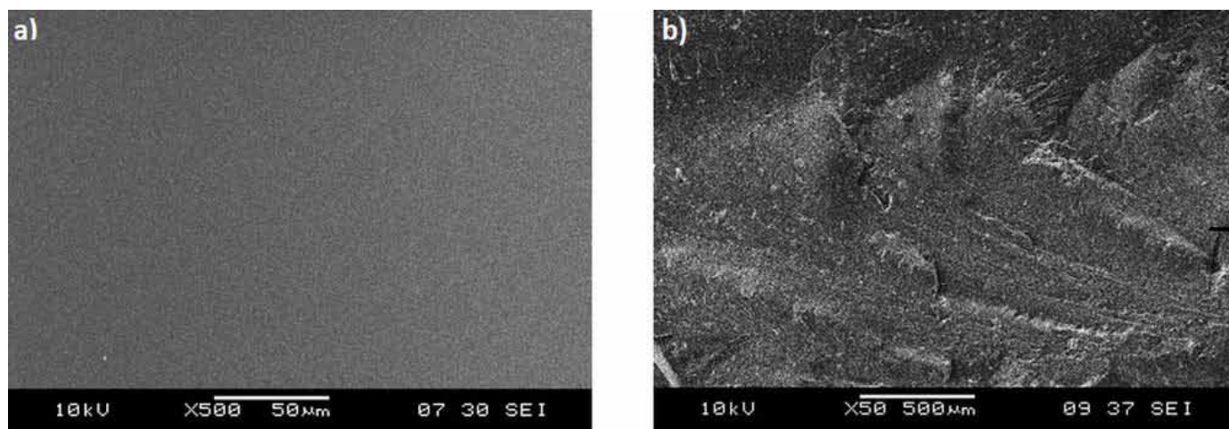
Fig. 8. SEM images of (a) DGEBA epoxy resin, (b) epoxy filled with fly ash-based geopolymer at 50× magnification
