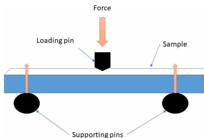
Fig. 2. The Illustration of Flexural Test
