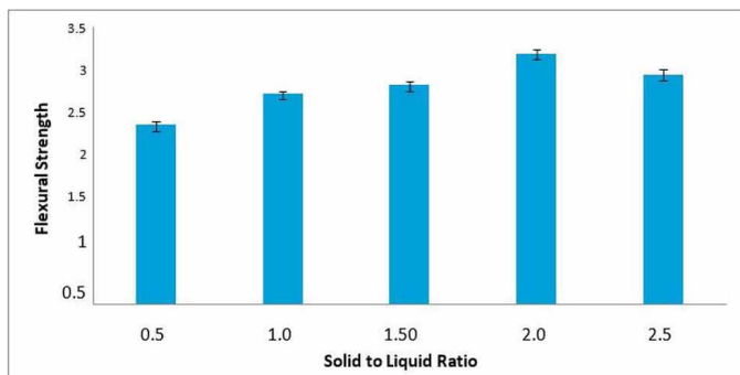
Fig. 5. Flexural Strength of Fly Ash-Based Geopolymer at Different Solid to Liquid Ratio
