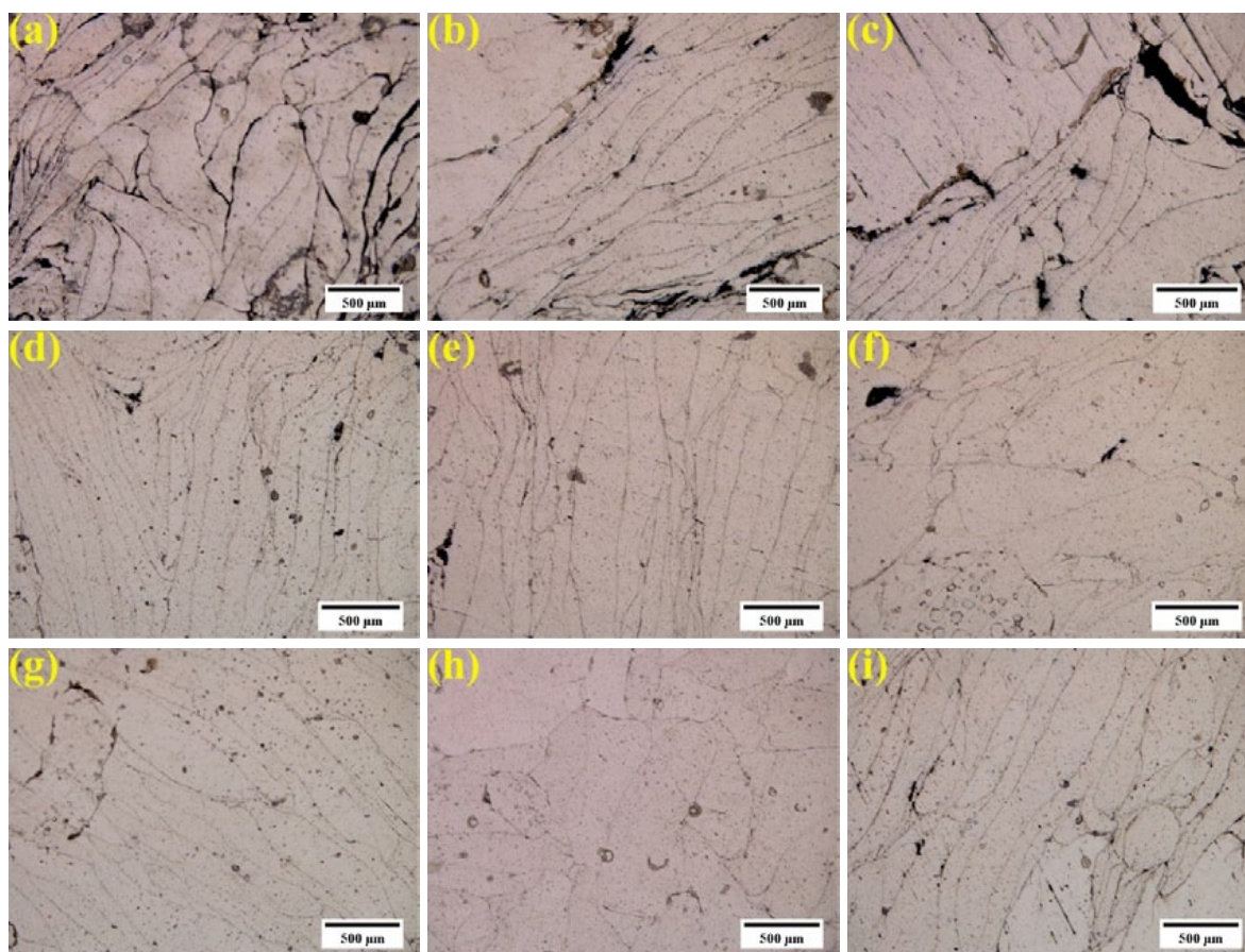
Fig. 14. Optical microstructure of consolidated chips for: (a) 0.4 mm DOC & 60°C CA, (b) 0.4 mm DOC & 75°C CA, (c) 0.4 mm DOC & 90°C CA, (d) 0.6 mm DOC & 60°C CA, (e) 0.6 mm DOC & 75°C CA, (f) 0.6 mm DOC & 90°C CA, (g) 0.8 mm DOC & 60°C CA, (h) 0.8 mm DOC & 75°C CA, (i) 0.8 mm DOC & 90°C CA
