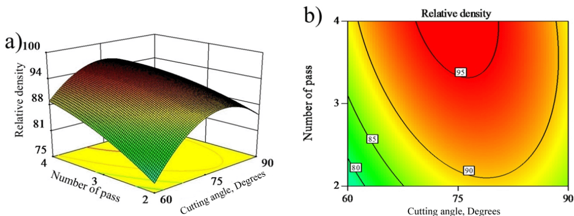
Fig. 17. Surface and contour plots representing the effect of number of passes and CA on relative density
