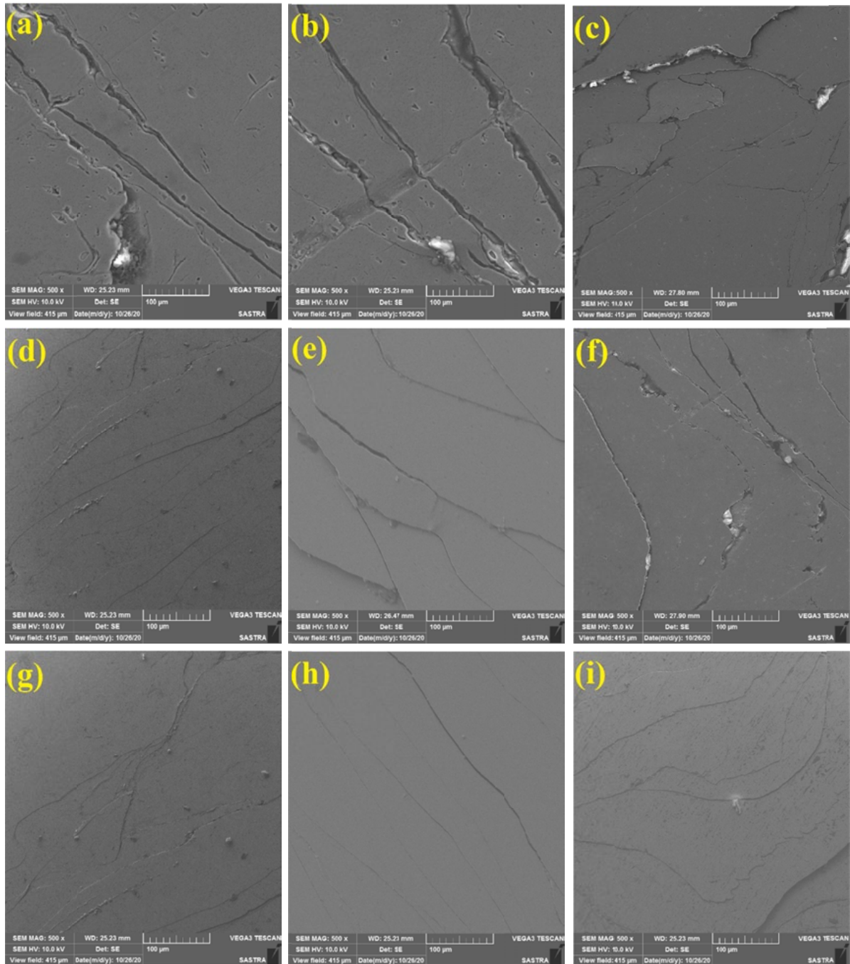
Fig. 15. Surface morphology of consolidated chips obtained by SEM for: (a) 0.4 mm DOC & 60°C A , (b) 0.4 mm DOC & 75°C A , (c) 0.4 mm DOC & 90°C A , (d) 0.6 mm DOC & 60°C A , (e) 0.6 mm DOC & 75°C A , (f) 0.6 mm DOC & 90°C A , (g) 0.8 mm DOC & 60°C A , (h) 0.8 mm DOC & 75°C A , (i) 0.8 mm DOC & 90°C A
