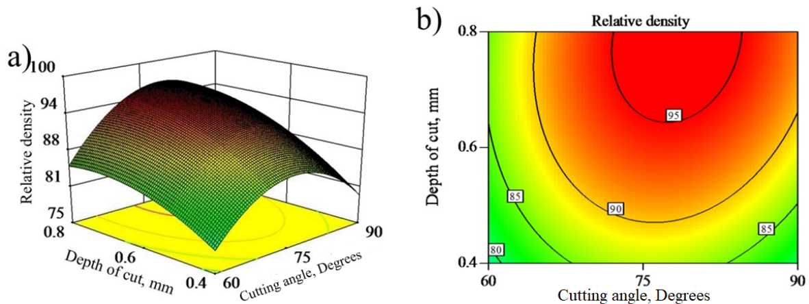
Fig. 16. Surface and contour plots representing the effect of DOC and CA on relative density
