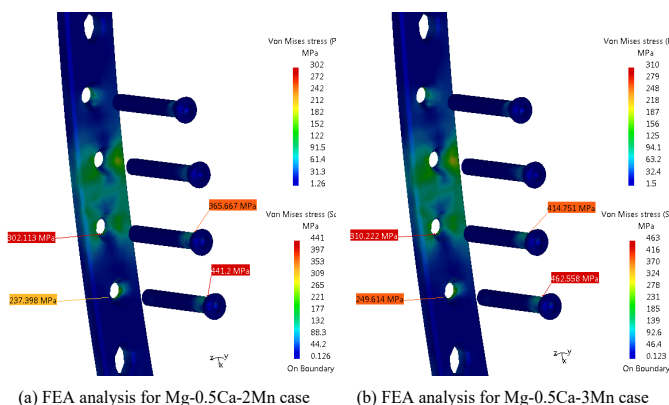
Fig. 4. Von Mises stress comparison between lower case (Mg-0.5Ca-2Mn case) and higher case (Mg-0.5Ca-3Mn case)
