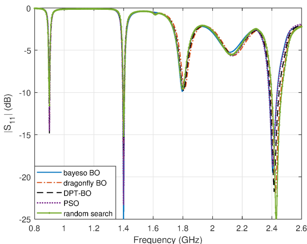
Fig. 5. Antenna S11 characteristics comparison
