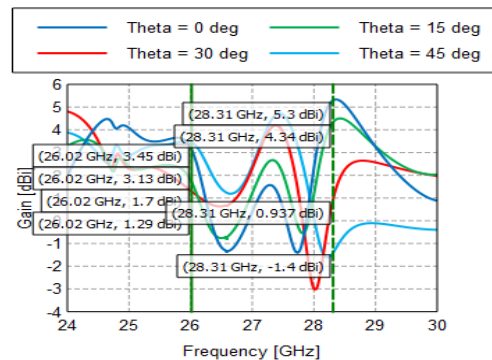
Fig. 20. Gain for 3 radiating elements with SRR
