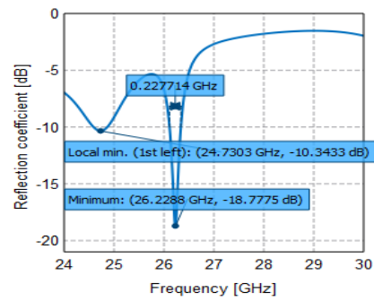
Fig. 8. Return loss and bandwidth. Impedance matching characteristic
