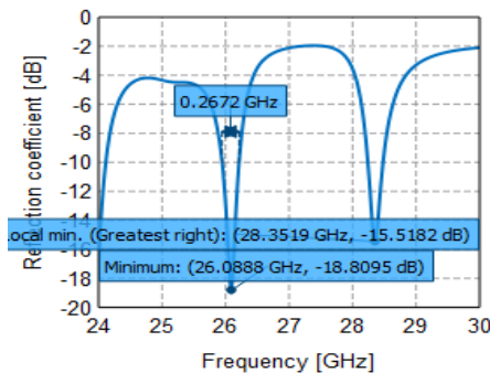
Fig. 13. Return loss and bandwidth of 2 radiating elements with SRR
