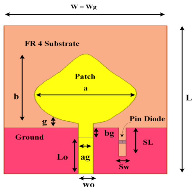
Fig.2. Proposed Antenna Design
