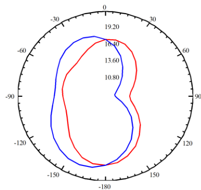
Fig.10. Radiation pattern of PIN Diode OFF Condition
