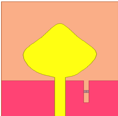
Fig.7. Design of Proposed structure
