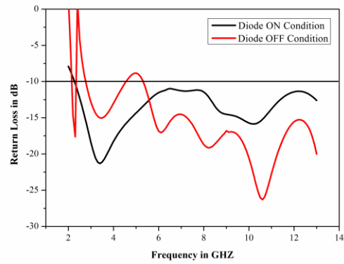
Fig.8. Return Loss curve for Design 4 in ON & OFF Conditions
