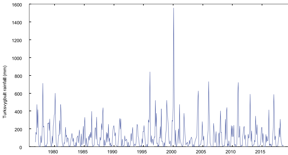
Fig. 1. Time series plot of the Turksygbult rainfall from 1976 to 2018; source: own study
