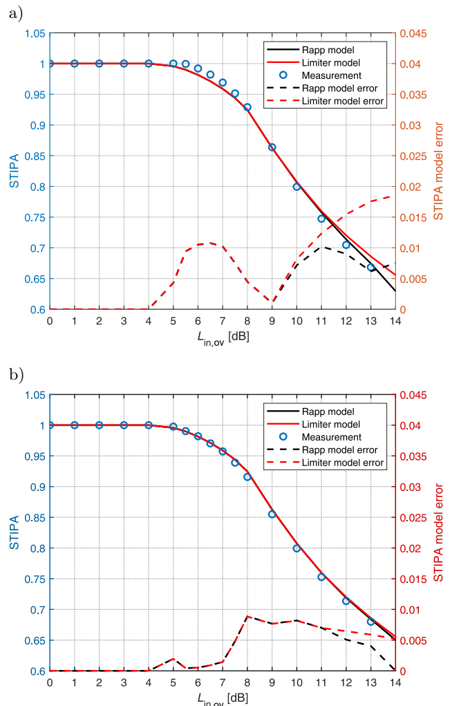
Fig. 4. Effect of the amplifier on STIPA obtained by modelling compared with measured results for: a) Class AB, b) Class D.
