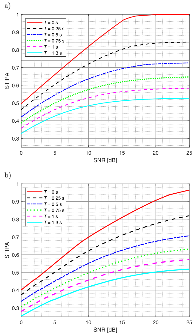
Fig. 6. Effect of signal-to-noise ratio on STIPA for an ideal amplifier and selected values of reverberation time, signal level L_{Aeq,s} = 75 dB and two interfering noise spectra: a) male speech, b) pink noise.
