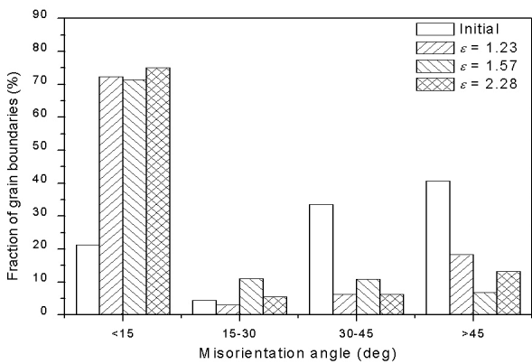
Fig. 6. Angles of grain disorientation in the CuCrZr copper alloy in the initial state and after the hydrostatic extrusion process
