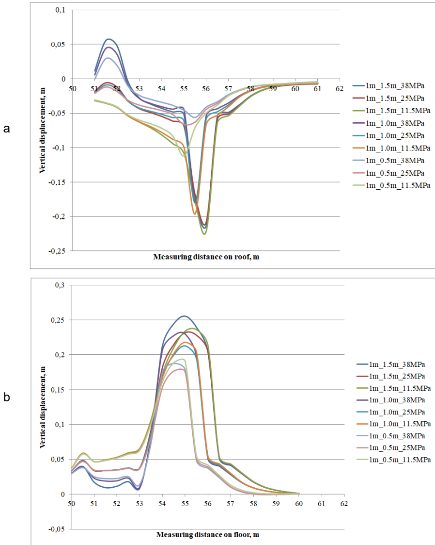
Fig. 13. Vertical displacement around the longwall face in the case of 1.0 m thick of shale with coal lamina: a) roof; b) floor
