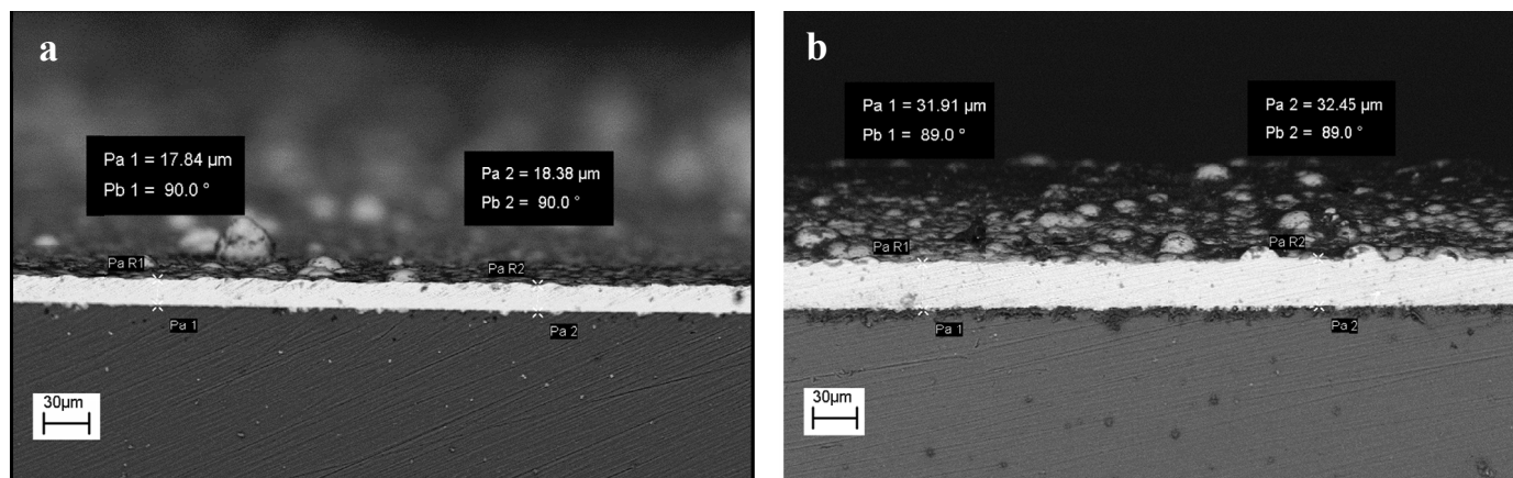
Fig. 3. The cross-sectional view of the electroless Ni-P coating on Ti/Zr (a) and Ti-Zr/sol-gel (b)
