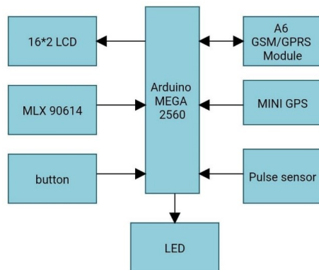
Fig. 1. The block diagram of the soldier mobile unit
