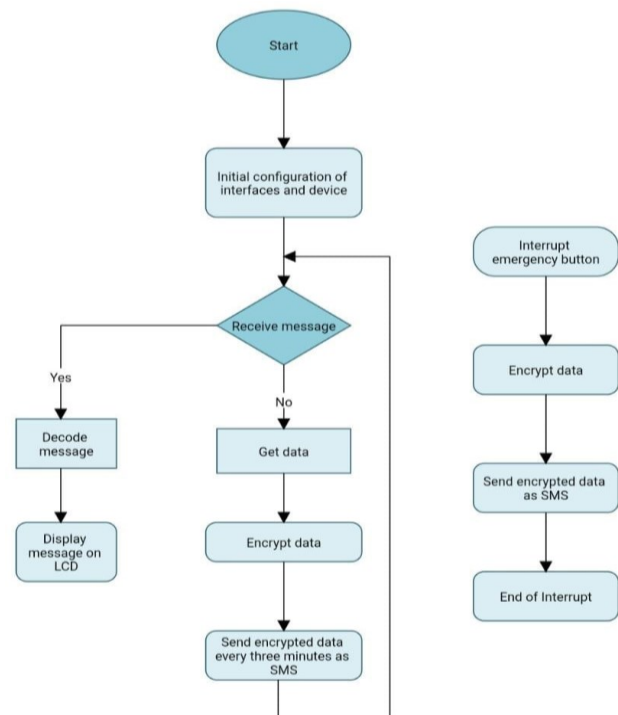
Fig. 3. Flow chart diagram of the soldier mobile unit
