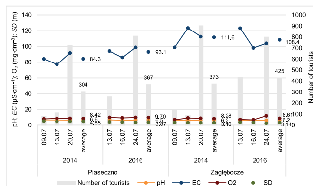
Fig. 6. Daily and average seasonal values of physical and chemical water parameters: reaction (pH), electrolytic conductivity (EC, in µS·cm -1 ), oxygen concentration (O 2 , in mg·dm -3 ), and water transparency as Secchi disk visibility (SD, in m) for Lakes Piaseczno and Zagłębcze in the summer of 2014 and 2016 in relation to the number of tourists; source: own study
