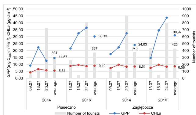
Fig. 5. Daily and average seasonal values of biological trophic state indices: gross primary production of phytoplankton (GPP, in mg C ass ·m -3 ·h -1 ) and chlorophyll a concentration (CHLa, in µg·dm -3 ) for Lakes Piaseczno and Zagłębcze in the summer of 2014 and 2016 in relation to the number of tourists; source: own study
