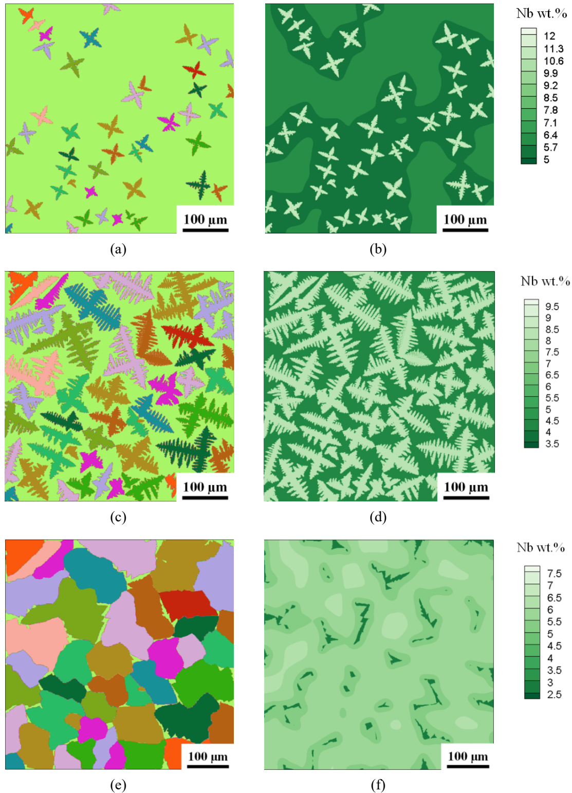
Fig. 4. Simulated dendrite microstructures (a, c, and e) and corresponding Nb concentrations (b, d, and f) of the U-5.5Nb alloy during solidification, where t = 1.9 s, 6.7 s, and 12.4 s, respectively
