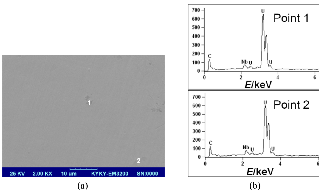
Fig. 3. SEM morphology of inclusions (a) and EDS results (b) of points 1 and 2
