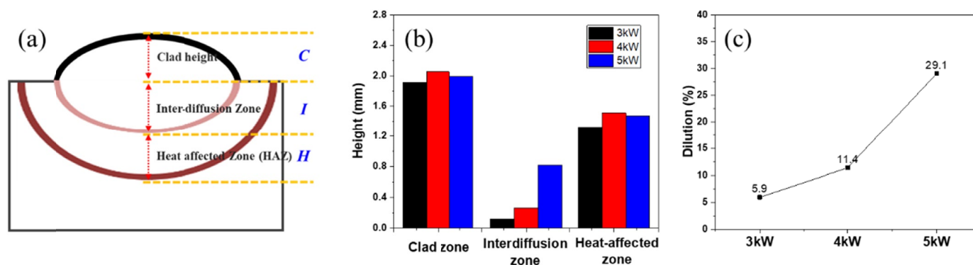
Fig. 1. The cross-sectional image of laser-clad specimen (a) showing distinct three areas – (1) clad, (2) interdiffusion, and (3) heat affected zone – coating height (b) corresponding to distinct area (a), and dilution rate (c) with various laser powers, 3, 4, 5 kW
