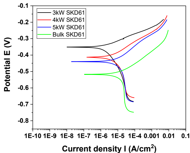
Fig. 4. Polarization curves of specimens after potentiodynamic test in NaCl solution at 25°C
