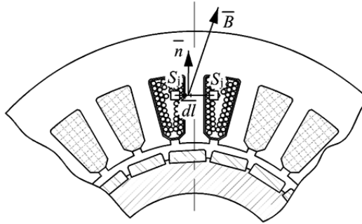
Figure 2: To calculate the total flux linkage of the coil
