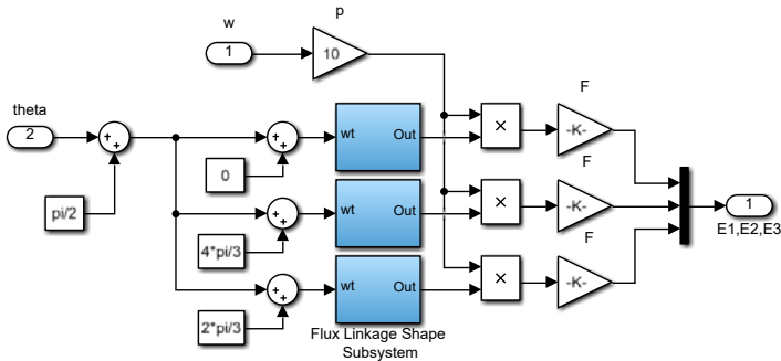
Figure 14: Computer model of the EMF Subsystem for one machine module
