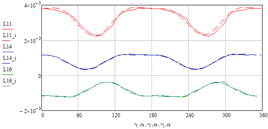
Figure 11: Comparison of the related to phase 1 angular dependencies of self and mutual inductances (solid lines) with their approximated by (15) functions (dashed lines)
