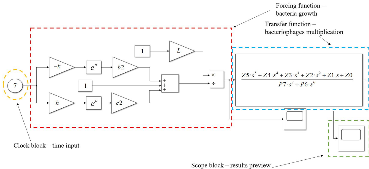
Fig. 4. Dynamic model structure created in Matlab and Simulink software representing Eq. (6) and Eq. (10)
