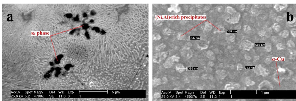
Fig. 6. SEM micrographs showing a) \kappa_1 intermetallic phase formed and uniform distribution, b) of Al-rich precipitates in the alloyed zone of SA130-30-1 specimen
