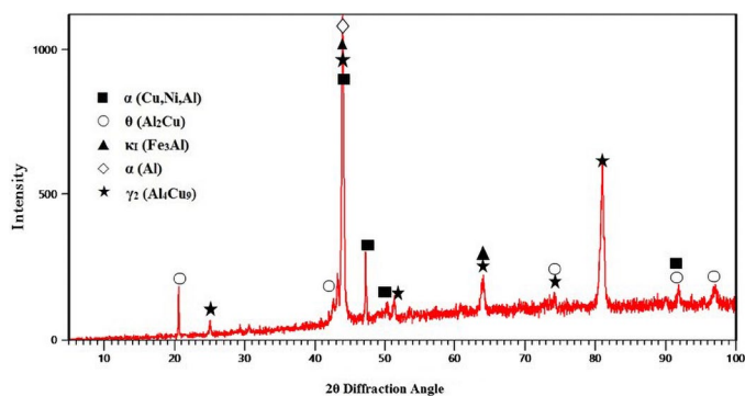
Fig. 5. XRD pattern of the surface alloyed specimen (SA130-30-1) achieved by 1.87 kJ/mm heat input
