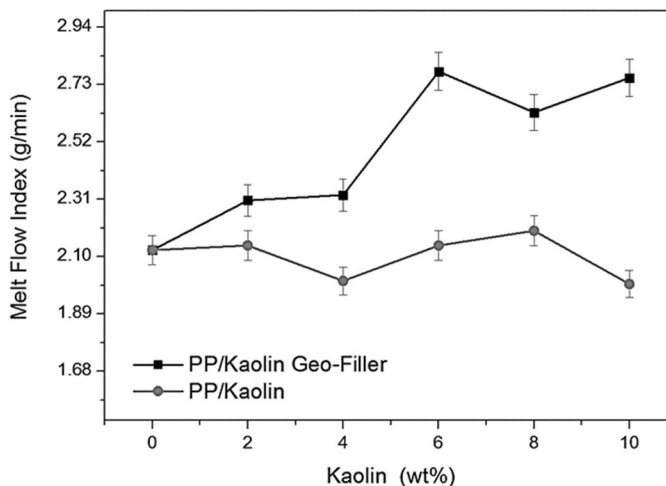
Fig. 1. PP composites melt flow index variations as a function of raw kaolin and kaolin geo-filler concentration
