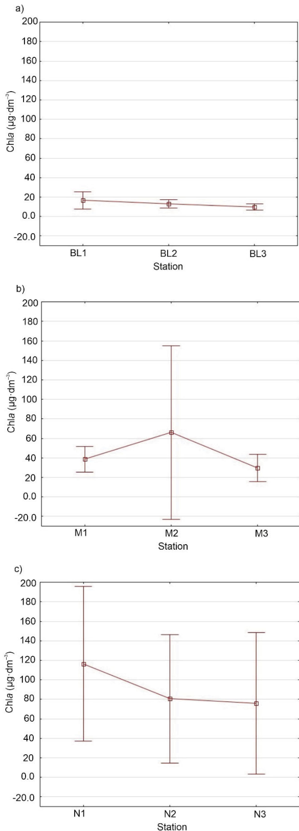
Fig. 3. Distribution of mean values (with confidence intervals) of Chla in waters of the studied reservoirs: a) Blizne, b) Maziarnia, c) Nielisz; source: own study
