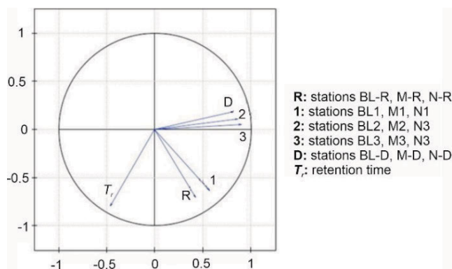
Fig. 5. Results of principal component analysis (PCA); the effect of water retention time ( T_r ) in the reservoirs on the concentration of organic matter ( OM_{SS} ) contained in suspended sediment (SS); source: own study
