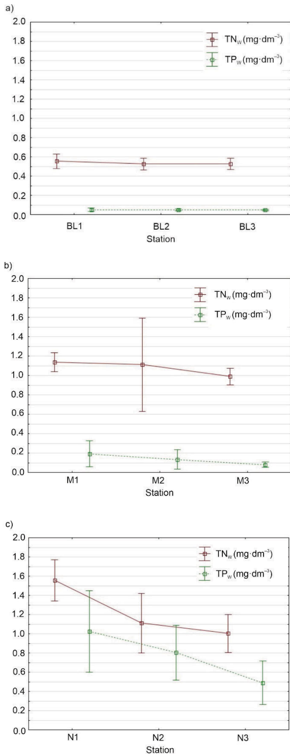
Fig. 2. Distribution of mean concentrations (with confidence intervals) of total phosphorus (TP w ) and total nitrogen (TN w ) in waters of the studied reservoirs: a) Blizne, b) Maziarnia, c) Nielisz; source: own study
