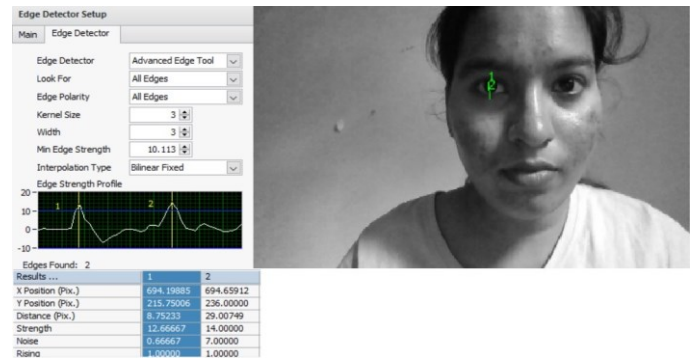
Fig. 25. Vision Assistant module for detecting Edges
