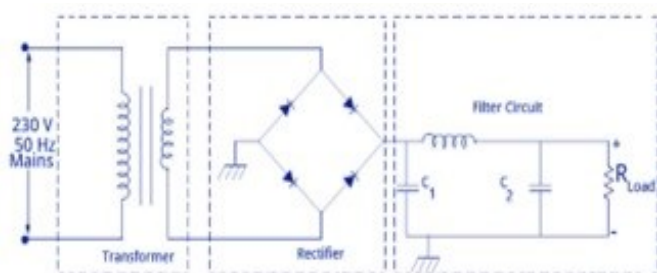
Fig. 7. Power Supply
