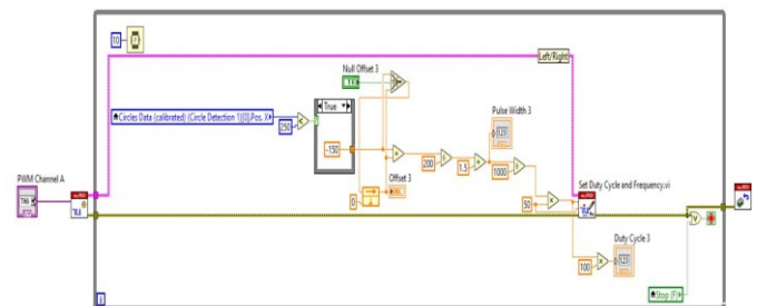
Fig. 19. Block diagram for Servo motor Left/Right rotation
