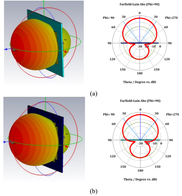
Fig. 13. Farfield radiation pattern of (a) Design C – Denim Textile and (b) Design C – Polyester Fabric
