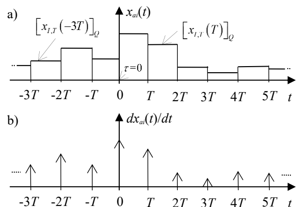
Fig. 6. Sketches illustrating forms of the waveforms: a) of the ideal version of x_a(t) called here x_{ai}(t) , and of the derivative of the latter.
