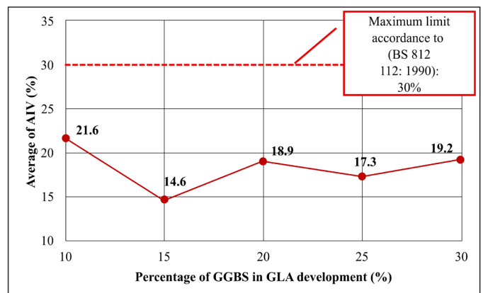
Fig. 5. Aggregate Impact Value (AIV) of GLA
