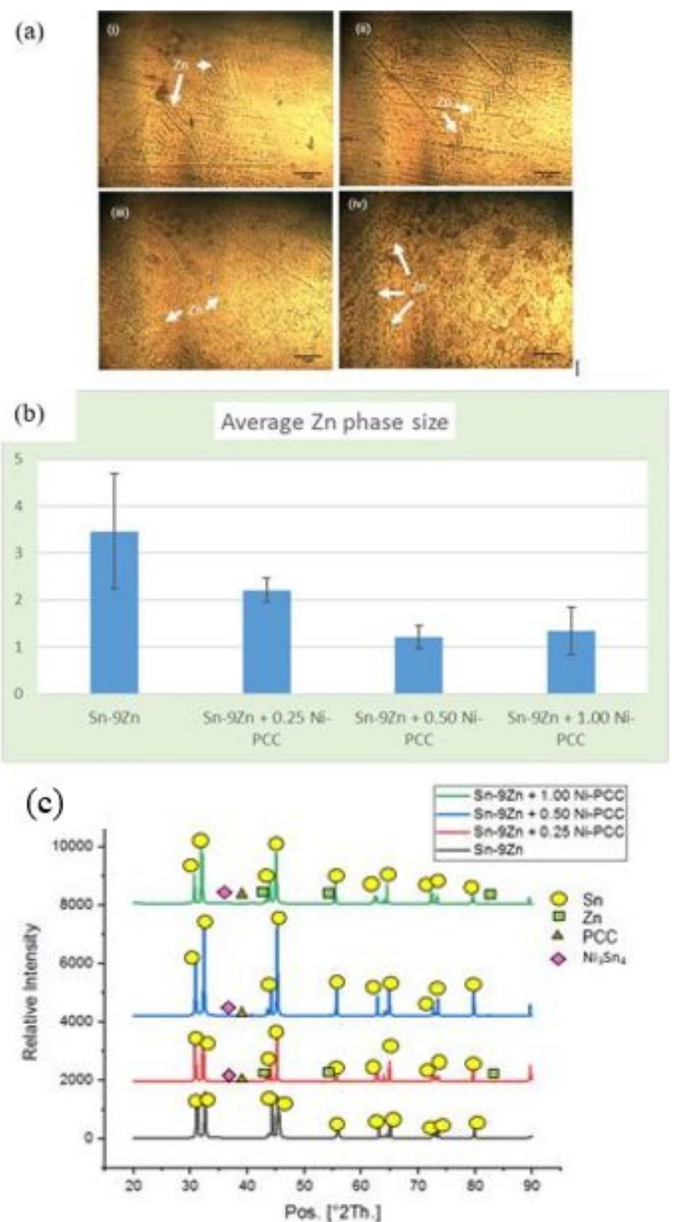
Fig. 3. (a) Microstructure of composite solder Sn-9Zn + xNi-PCC (i) x = 0, (ii) x = 0.25, (iii) x = 0.50, (iv) x = 1.00 wt.%; (b) Average size of Zn phase of composite solder Sn-9Zn + xNi-PCC (x = 0, 0.25, 0.50 & 1.00 wt.%)
