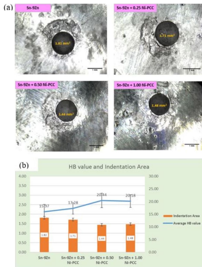
Fig. 5. (a) Image of indentation of composite solder Sn-9Zn + xNi-PCC ( x = 0.25, 0.50 & 1.00 wt.%) after Brinell Test; (b) Average HB value and Indentation Area of composite solder Sn-9Zn + x Ni-PCC ( x = 0.25, 0.50 & 1.00 wt.%) after Brinell Test
