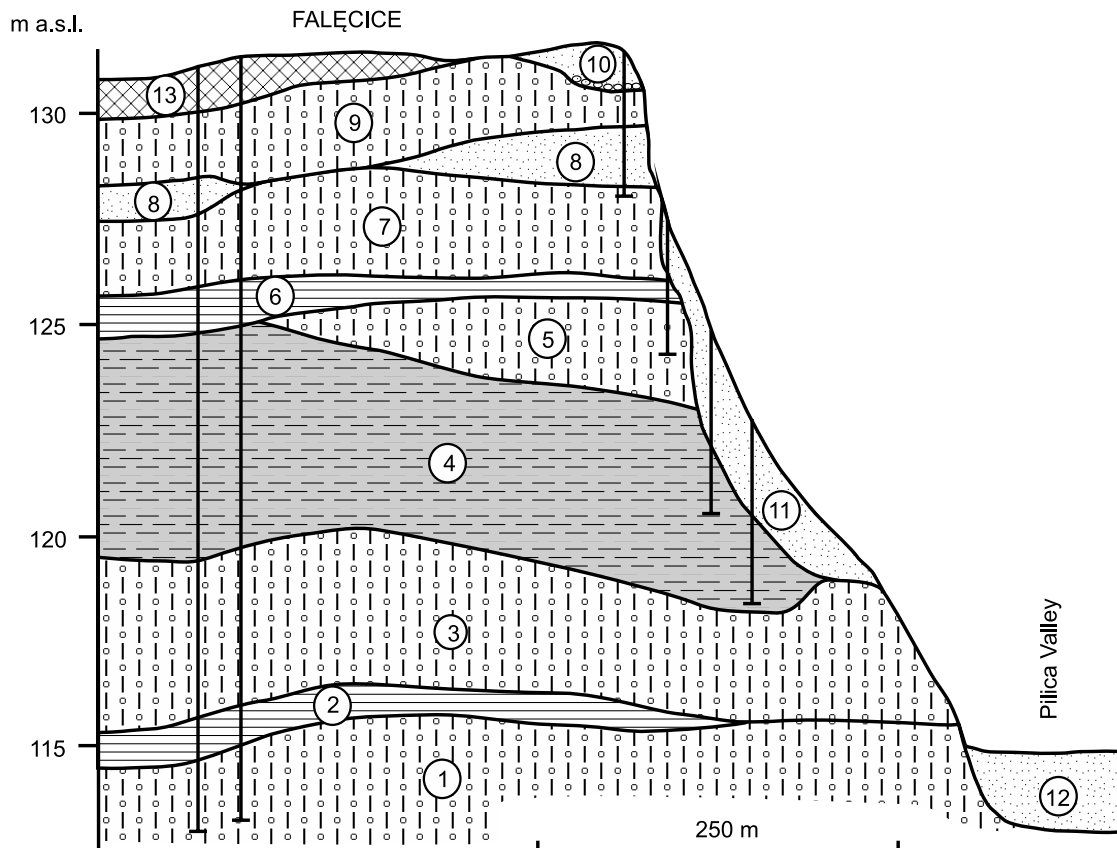
Text-fig. 4. Geological position of deposits representing the Ferdynandovian Interglacial in Falęcice (after Lindner et al. 1991a and unpublished data). Nidanian Glaciation: 1 – glacial till; 2 – ice-dammed lake silt; Sanian 1 Glaciation: 3 – glacial till; Ferdynandovian Interglacial: 4 – lake clay with peat intercalations and shaly clay; Sanian 2 Glaciation: 5 – glacial till; Krznanian (?) Glaciation: 6 – ice-dammed lake silt; 7 – glacial till; Lubavian Interglacial: 8 – fluvial sand and gravel; Odranian Glaciation: 9 – glacial till; 10 – glaciofluvial sand and gravel; Vistulian glaciation: 11 – slopewash deposits; 12 – fluvial sand; Holocene: 13 – anthropogenic material.
