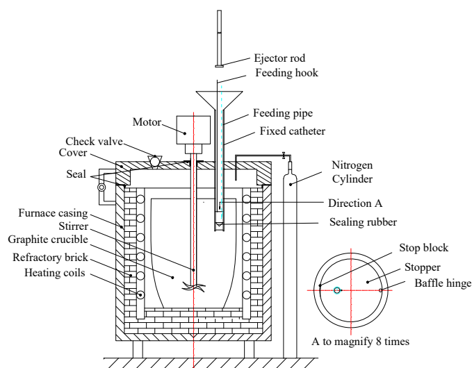
Fig. 2. Schematic diagram of composite material preparation equipment
