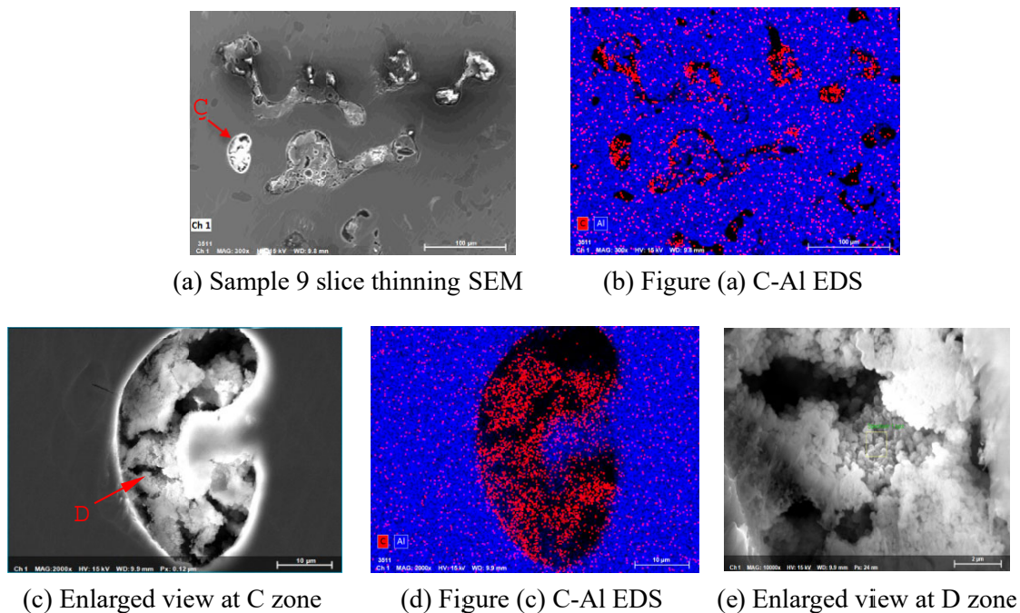
Fig. 12. SEM image and EDS image of sample 9 slice thinning
