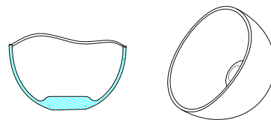
(b) Sample 9 “Eggshell”-shaped dimple model diagram
