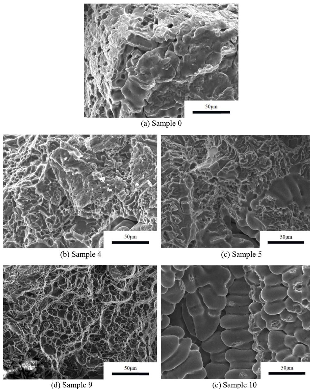
Fig. 8. SEM image of the fracture surface of ZL105 aluminum alloy reinforced with different aspect ratios and content of carbon nanotubes
