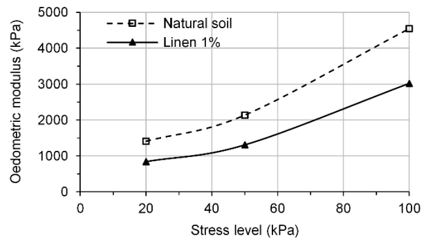
Fig. 6. Oedometric stiffness modulus as a function of the stress level; source: own study
