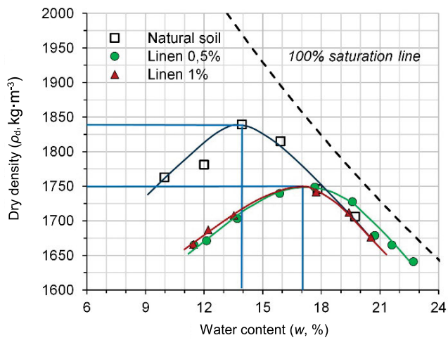
Fig. 4. Standard Proctor tests on natural soil ( w_{opt} = 14\% , \rho_{d,max} = 1840 kg·m -3 ) and treated soil ( w_{opt} = 17\% , \rho_{d,max} = 1750 kg·m -3 ); source: own study
