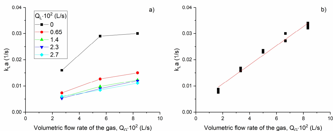
Figure 3. Volumetric mass transfer coefficients in a) Biostat PBR-2S (Sartorius) and b) Labfors 5 Lux LED (Infors HT).
