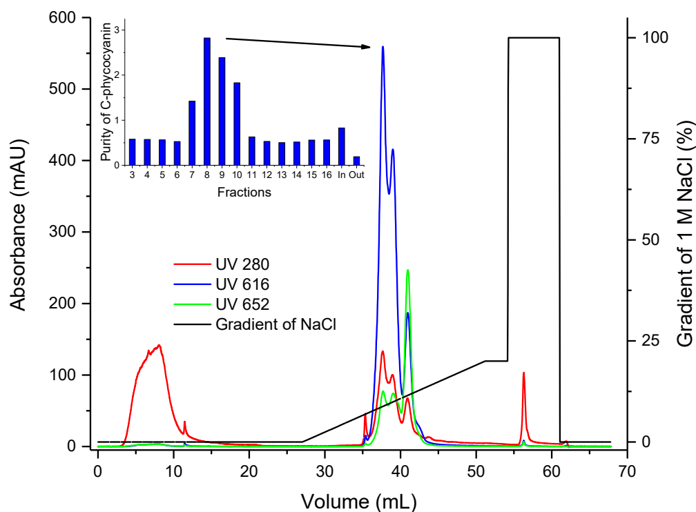
Figure 5. Purification of C-phycoerythrin by anion exchange chromatography on a Resource Q column.
