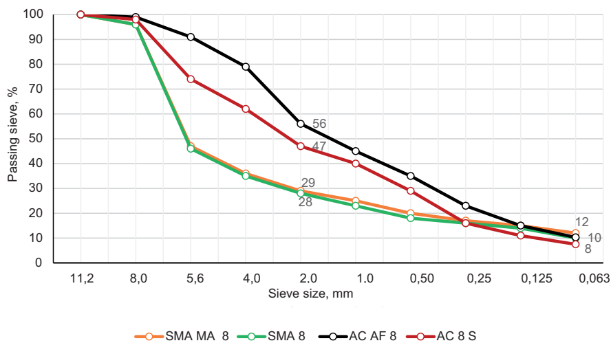
Fig. 4. Gradation curves of the tested mixtures
