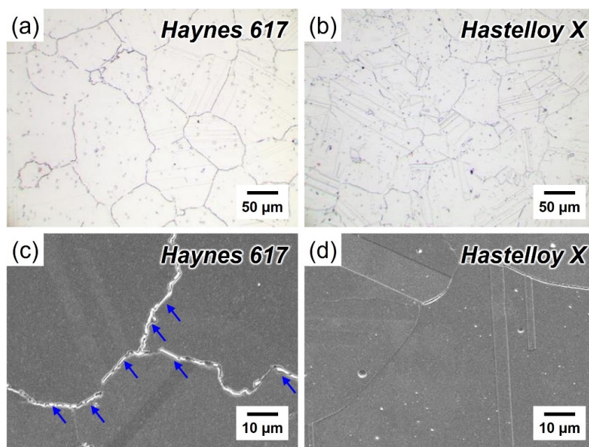
Fig. 2. (a) and (b) Optical microscope (OM) and (c) and (d) scanning electron microscope (SEM) micrographs of the Ni-based superalloys: (a) and (c) Haynes 617 alloy and (b) and (d) Hastelloy X alloy. The blue arrows indicate the presence of precipitates at grain boundaries of the Haynes 617 alloy. The grain size of the Haynes 617 and Hastelloy X alloys was measured to be 118.5 ± 5.1 μm and 66.2 ± 3.2 μm, respectively
