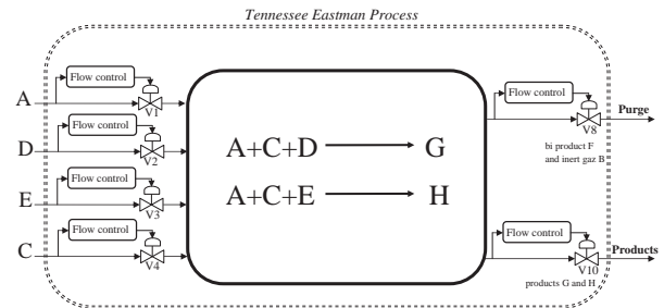
Fig. 4. General sketch of the TEP
