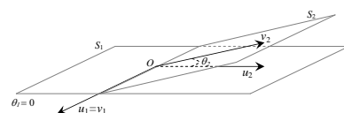
Fig. 2. Angle \theta_2 between the subspaces S_1 and S_2
