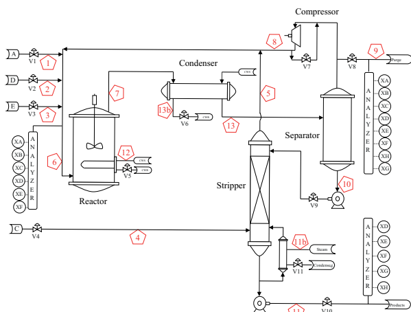
Fig. 5. Detailed layout of the TEP
