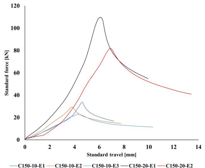
Fig.8. A) Load-displacement curves for different considered eccentricities
