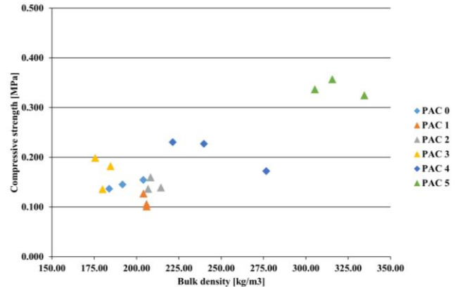
Fig.5. PAC compressive strength vs bulk density
