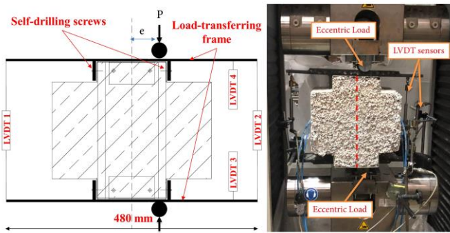
Fig.6. Zwick Z400 universal machine and sensor locations
