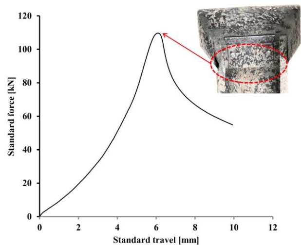
Fig.9. Test data for C150-20-300-E1 (Load-displacement curve)
