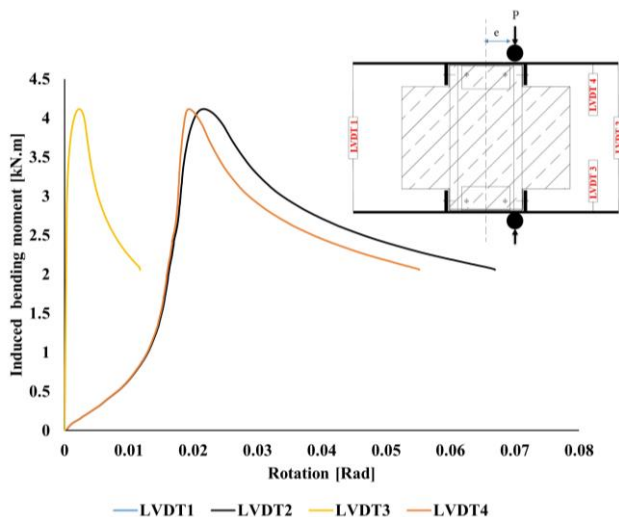
Fig.10. Test data for C150-20-300-E1 end joint rotation
