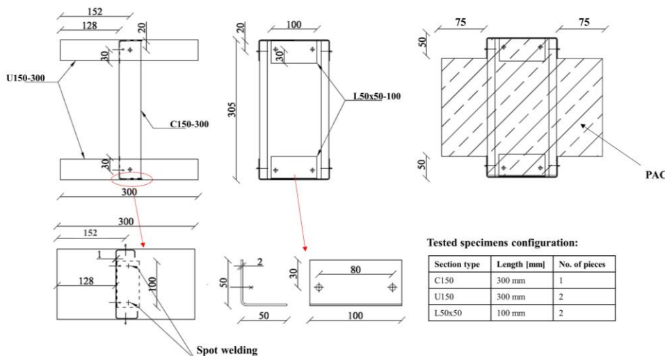
Fig.3. Tested C-section details
