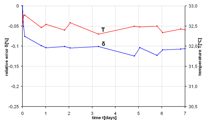
Fig. 4. Relative error of VW strain gauge relaxation (Fig. 2) after step application of deformation corresponding to a change in the tension of the wire by approx. 60% of the rated measuring range
