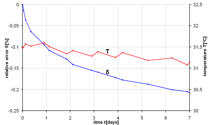
Fig. 3. Relative error of VW strain gauge relaxation (Fig. 2) after step application of deformation corresponding to a change in the tension of the wire by approx. 120% (still permissible) of the rated measuring range
