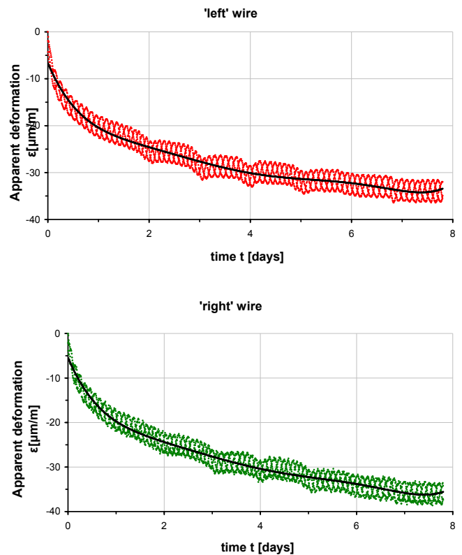
Fig. 10 The first part of the strain gauge test. Movable anchor in neutral position, both wires stresses equal
