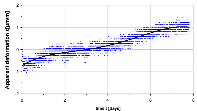
Fig. 11. Conditions as for Fig. 10, differential strain of the strain gauge and relaxation error
