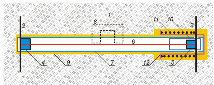
Fig. 7. A simplified scheme of the author's construction strain gauge for measuring deformation of a concrete structure. 1 – concrete mass, 2, 3 – anchors, 4, 5 – wire clamps, 6 – wire, 7 – housing, 8 – electromagnet, 9 – flexible coating, 10 – sliding sleeve, 11 – pre-tension spring, 12 – yoke
