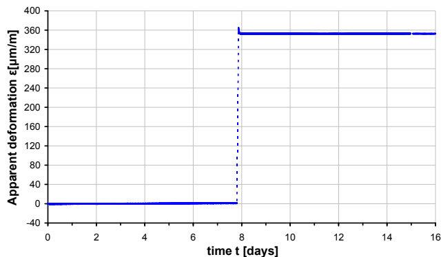
Fig. 16 Total deformations measured by the differential gauge during both parts of the test. The influence of the wire memory effect on the measurement results has been slightly reduced
