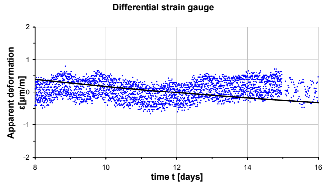
Fig. 14. Deformations measured by the differential gauge and its relaxation errors
