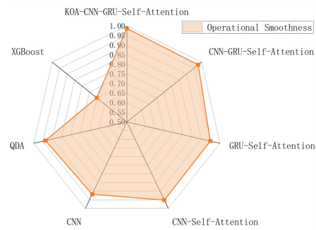
Fig.11. Comparison of accuracy of operational smoothness
