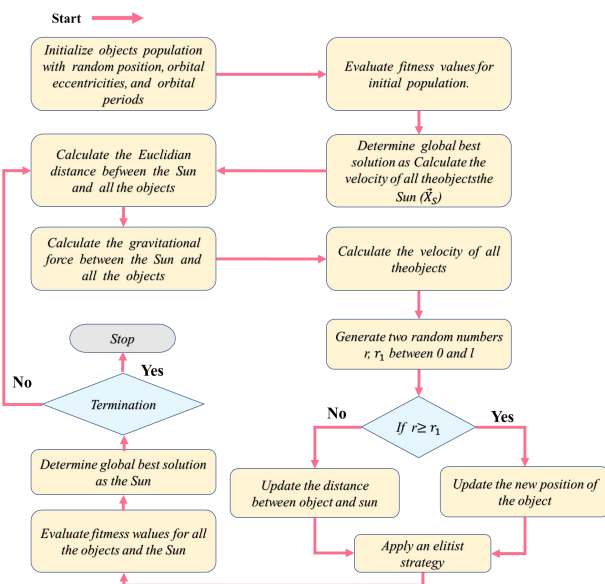
Fig.4. KOA Optimization Flowchart
