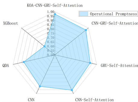
Fig.13. Comparison of accuracy of operational promptness
