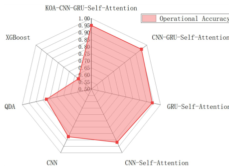
Fig.12. Comparison of accuracy of operational accuracy
