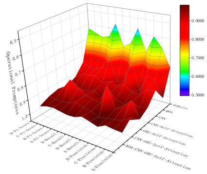
Fig.15. Comparison of precision&recall&F1-score of operational accuracy
