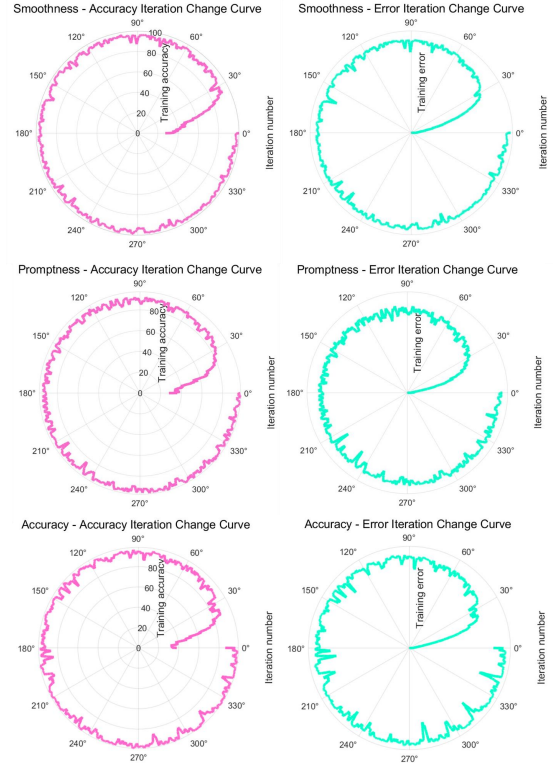
Fig.7. Iteration change curve of Accuracy & Error
