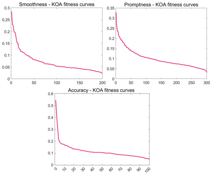
Fig.6. KOA fitness curves
