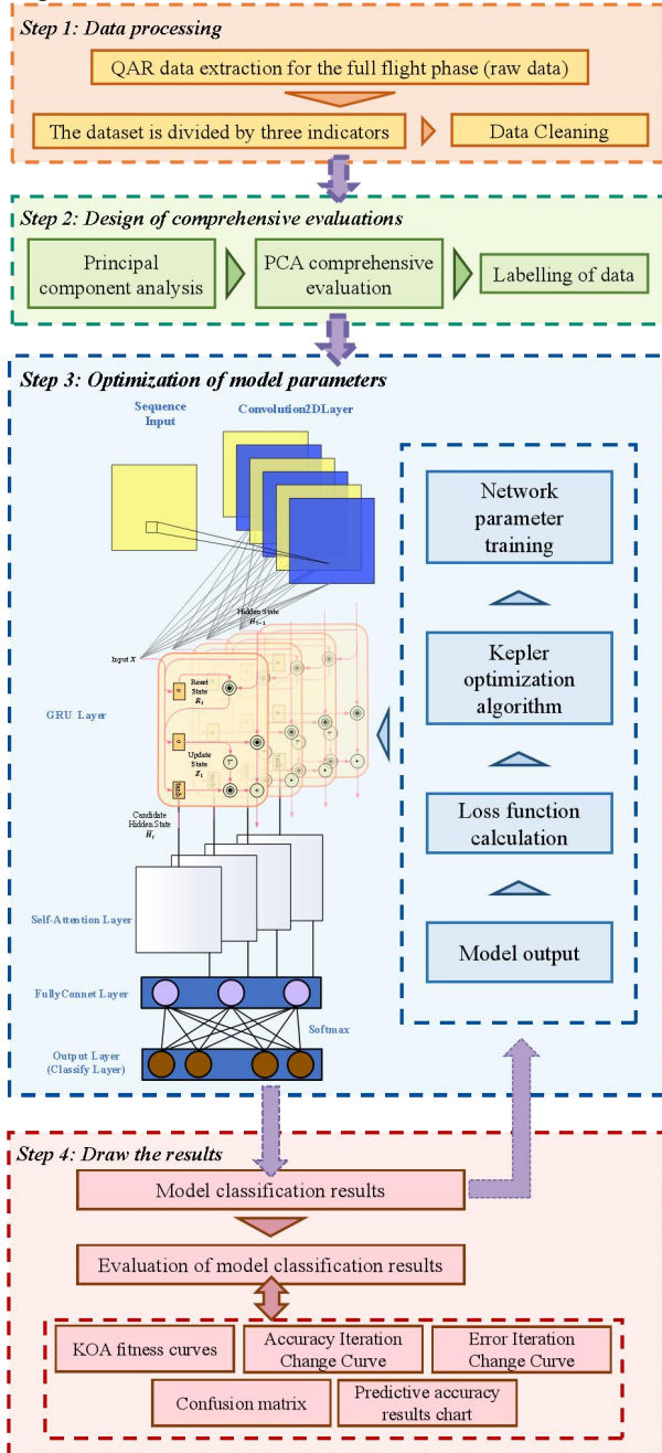
Fig.1. Training process of KOA-CNN-GRU-Self-Attention model
