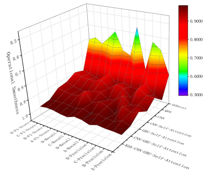
Fig.16. Comparison of precision&recall&F1-score of operational promptness
