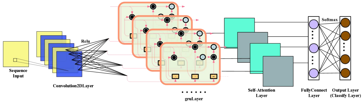
Fig.5. CNN-GRU-Self-Attention model
