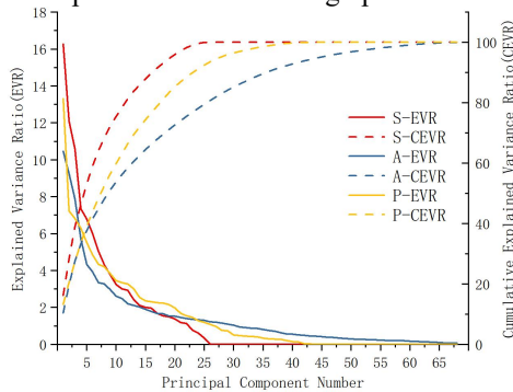
Fig.3. Plot of explained variance by principal components
