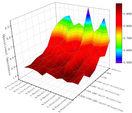
Fig.14. Comparison of precision&recall&F1-score of operational smoothness
