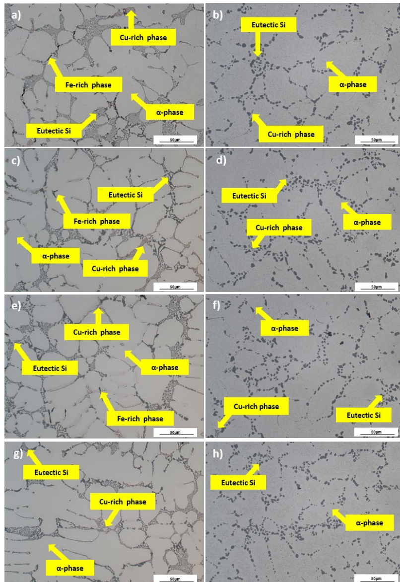
Fig. 7. Microstructural evaluation of experimental alloys in as-cast state and after heat treatment T6: a) Ref. alloy/AC; b) Ref. alloy/T6; c) R-Zr/AC; d) R-Zr/T6; e) R-Sr/AC; f) R-Sr/T6; g) R-Mo/AC; h) R-Mo/T6
