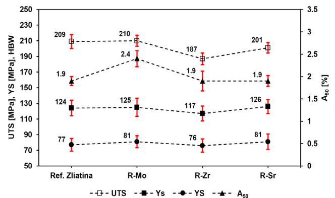
Fig. 2. Mechanical properties of experimental alloys in as-cast state [19]
