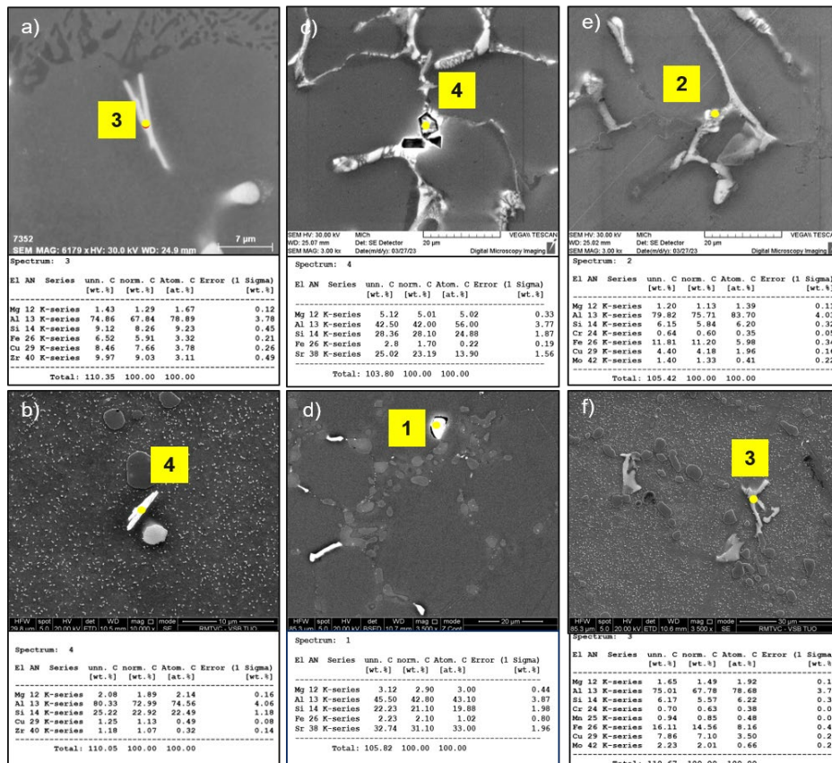
Fig. 8. EDX analysis of experimental alloys in as-cast state and after heat treatment T6: a) R-Zr/AC; b) R-Zr/T6; c) R-Sr/AC; d) R-Sr/T6; e) R-Mo/AC; f) R-Mo/T6
