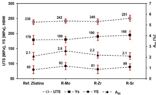
Fig. 3. Mechanical properties of experimental alloys after heat treatment T6
