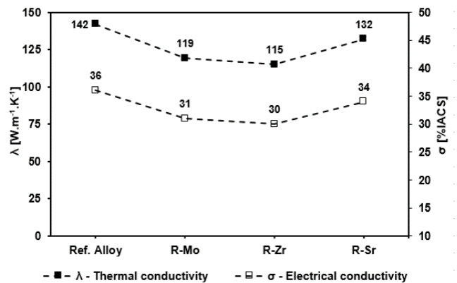
Fig. 4. Physical properties of experimental alloys in as-cast state [19]
