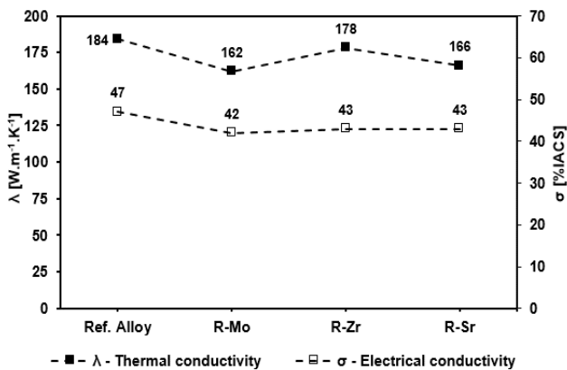
Fig. 5. Physical properties of experimental alloys after heat treatment T6
