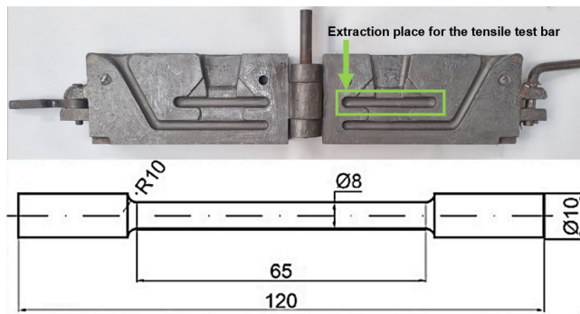
Fig. 1. Metal mold and scheme of tensile test bar
