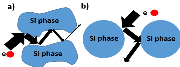
Fig. 6. Transfer of electrons: a) as-cast state; b) after heat treatment T6 [23]
