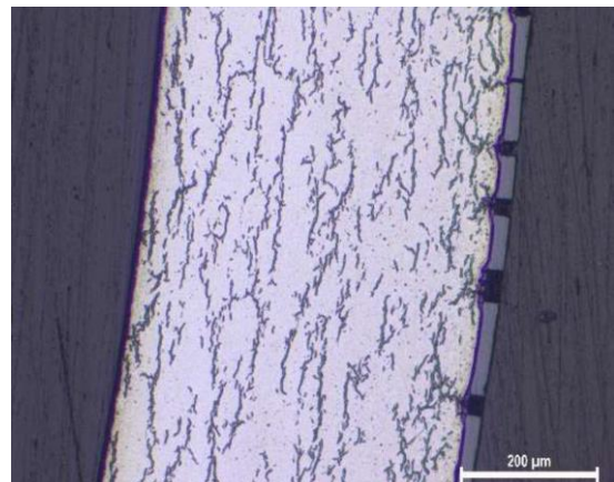
Fig. 1. The metallographic cross-section for E110 fuel cladding of 585 µm wall thickness [14].
