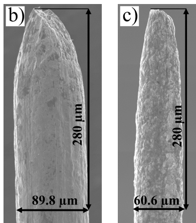
Fig. 11. The classic method of sharpening wires using stretching in a furnace: (a) graph of wire thickness after the sharpening process, (b) neck dimensions for Cu, (c) neck dimensions for the CuZn37 alloy
