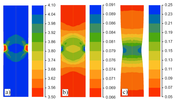
Fig. 10. Results of modelling incremental stretching of Cu wire: distribution of K (a) and effective strain (b, c) for the first strain increment lasting 100 ms (a, b) and the sixth increment of deformation (c)
