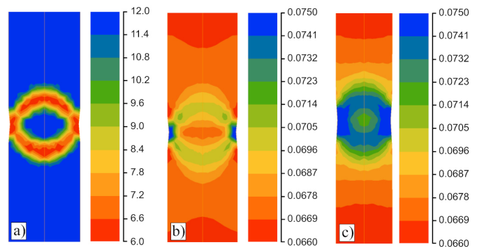
Fig. 9. Results of modelling incremental stretching of CuZn37 wire: distribution of K (a) and effective strain (b, c) for the first strain increment lasting 100 ms (a, b) and the sixth increment of deformation (c)
