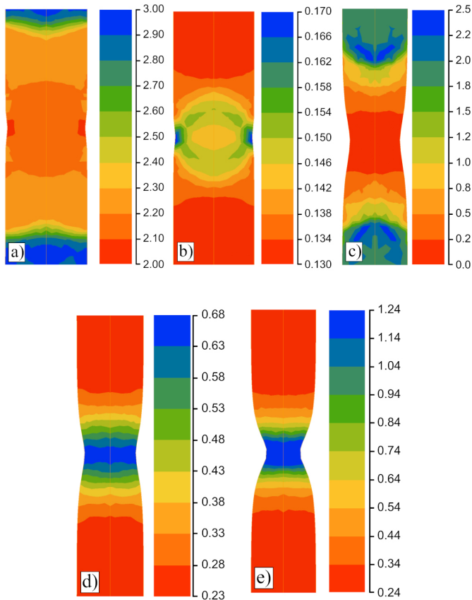
Fig. 8. Distribution of K (a, c) and effective strain (b, d, e) during the tension test of Cu wire at 200 ms (a, b), 400 ms (c, d), and 430 ms (e)
