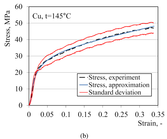
Fig. 5. The flow stress of the initial wire with a diameter of 0.1 mm: (a) CuZn37 alloy, (b) Cu
