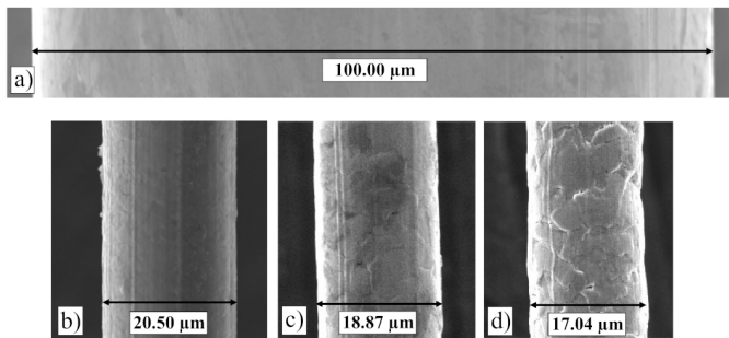
Fig. 13. CuZn37 wire: (a) input wire for the drawing process, (b) after the wire drawing process, (c) after sharpening using two passes of the IDD process, (d) after sharpening using four passes of the IDD process
