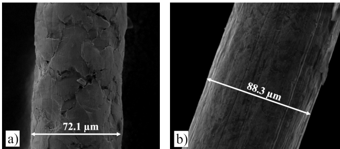
Fig. 12. Wire sharpening using the IDD technique for: (a) CuZn37, (b) Cu
