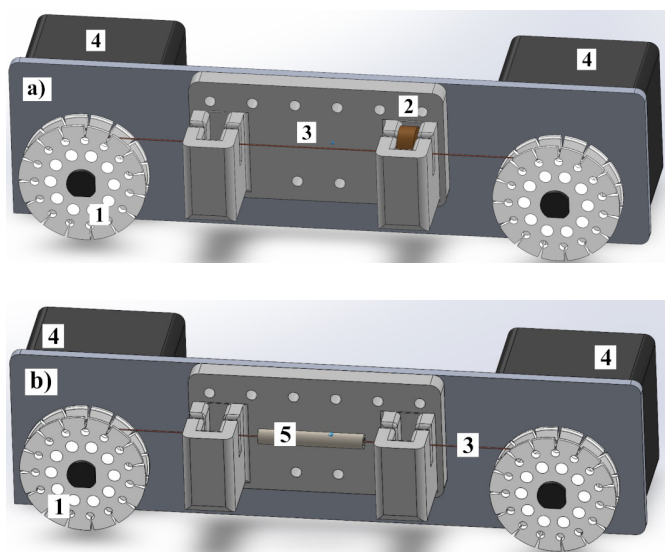
Fig. 4. Schematic of the machine for (a) drawing process and (b) sharpening process: 1 – uncoiler, 2 – drawing die, 3 – drawn wire, 4 – stepper motors, 5 – furnace
