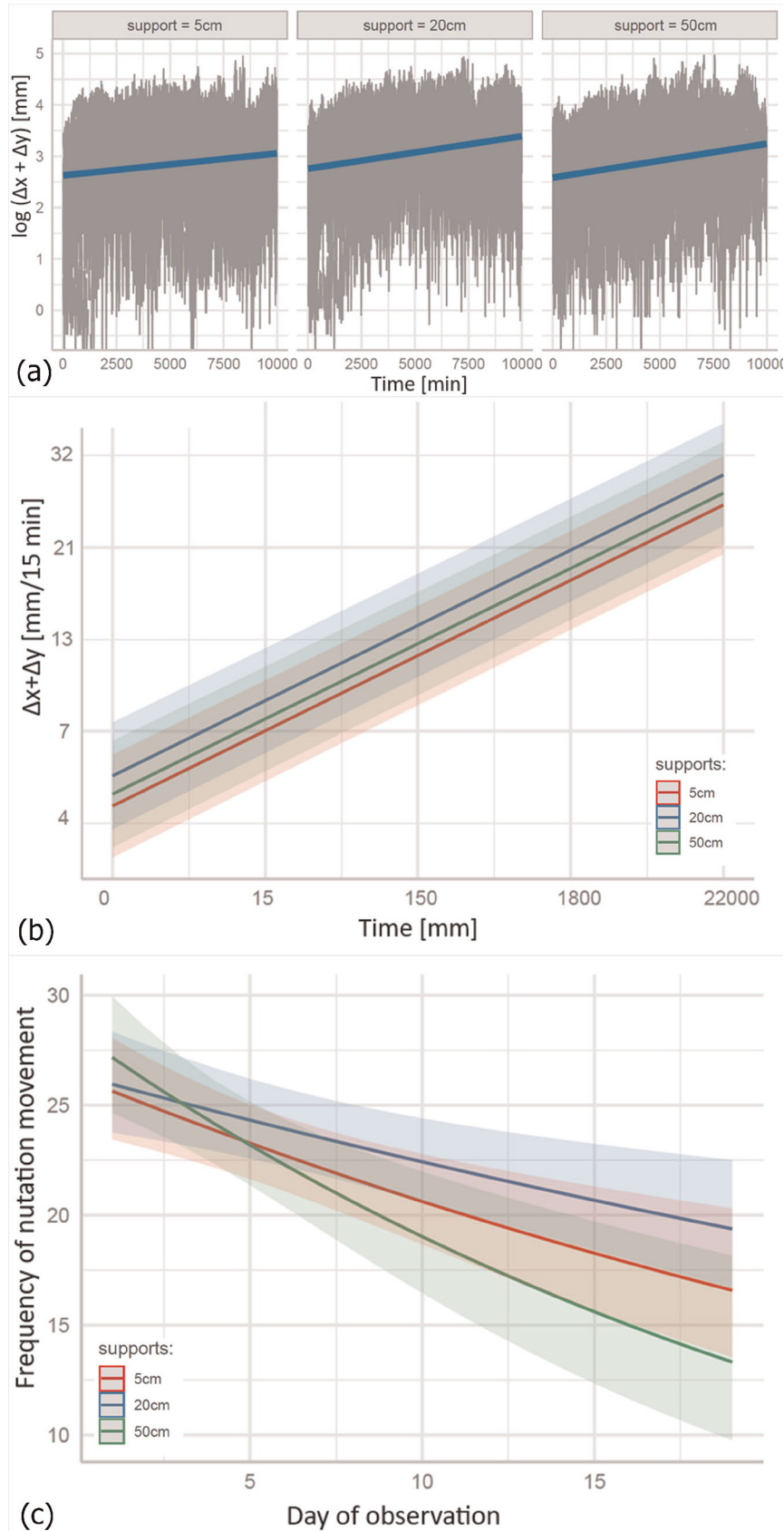
Fig. 2. (a) Illustration of temporal heterogeneity in plant apex deviation from the X- and Yaxes, by support group (5 cm, 20 cm, 50 cm) over a 0-10,000-minute time interval. The plant deviation trajectories are shown with the grey lines, emphasizing their unique growth patterns. The overarching deviation trends in each support group are captured by the blue lines, which represent the linear fit for each group, offering a simplified yet comprehensive view of the overall deviation tendencies. (b) Predicted plant apex deviation from the x and y axes as a function of time and supports variant, based on the fitted regression model (c) Predicted frequency of nutation movements as a function of the day of observation and support variants, based on the fitted regression model. (b) and (c) the opaque line indicates the midpoint of the interval, providing a central estimate of the growth rate. The 95% CI offered a range of plausible values for the frequency of nutation movements, indicating the uncertainty associated with the estimate.
