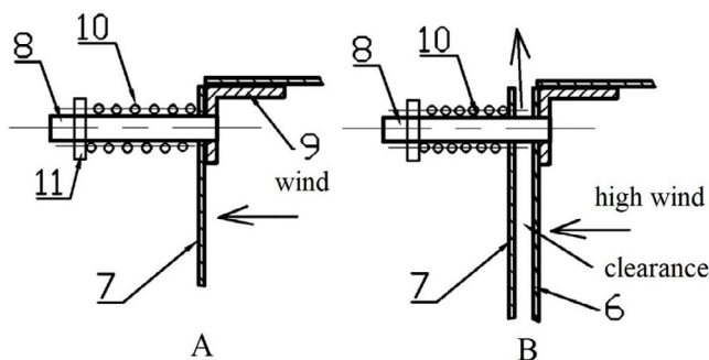
Fig. 7. Blade fragment with fixing rods and flap
