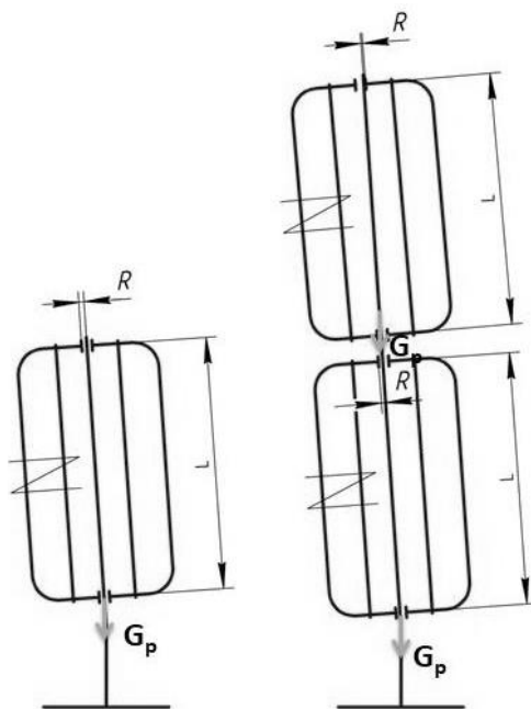
Fig. 4. Schemes of distribution of forces interfering with the operation of a wind turbine in a fixed axle design
