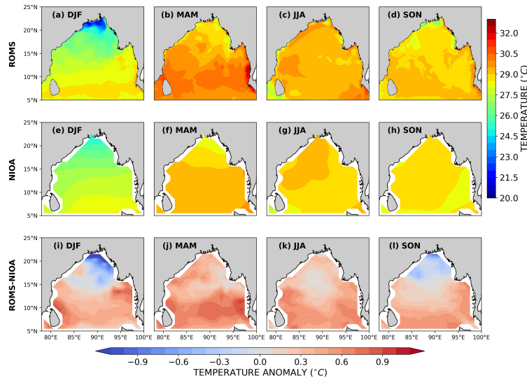
Figure 3. Spatial comparison of simulated ROMS SST (°C) in the first row, and observed NIOA SST (°C) in the middle row and the difference (ROMS-NIOA) in the lower row. Subplots a, b, c, and d represent ROMS SST for DJF, MAM, JJA, and SON seasons respectively. Subplots e, f, g, and h represent NIOA seasonal SST and subplots i, j, k, l represent the seasonal bias (ROMS-NIOA).
