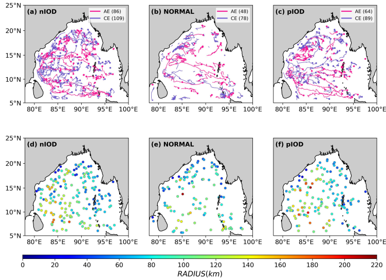
Figure 8. Subplots a, b, and c show the tracks for the negative IOD (nIOD) year, Normal year, and positive IOD (pIOD) year, respectively of the eddies in pink colour for Anticyclonic Eddy (AE), and blue colour for the Cyclonic Eddy (CE) having lifespan of at least 5 days. Dots show the eddy generation point and trails are the paths travelled by the eddies during their entire lifespan. Subplots d, e and f show the maximum radius attained by eddies during their entire lifespan for the corresponding eddies shown in subplots a, b, and c respectively. The magnitudes of the eddies' radius are given by the colour bar in km, the bubble size is uniform for all eddies.
