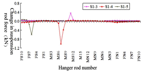
Fig. 13. S1-3~S1-5 Variation of boom force under damage condition
