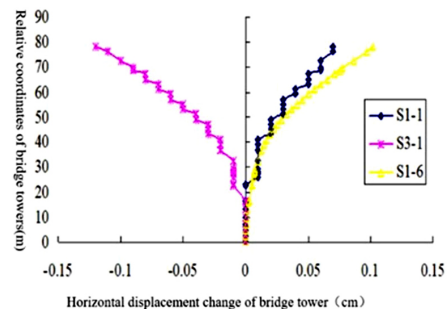
Fig. 8. Overall horizontal displacement change of bridge tower
