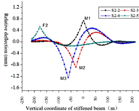
Fig. 10. Variation of deflection of main girder due to local damage of mid-span 1/4 span load
