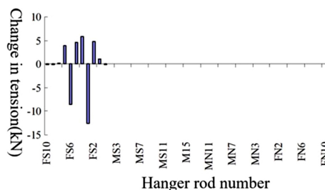
Fig. 32. Variation of lower boom force in combination 2
